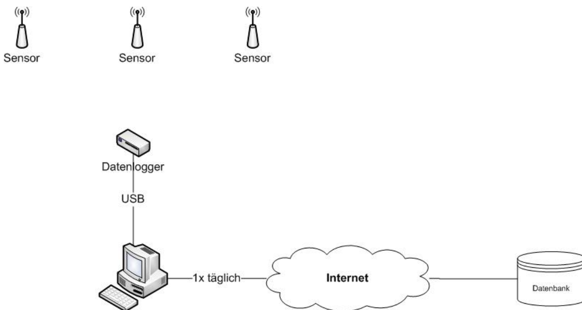
Figure 1: System Assembly
